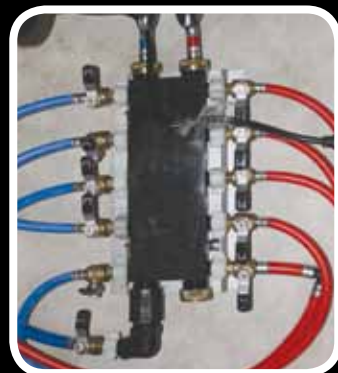
Water Manifold System improves flow and provides individual shut off for easy service or maintenance.
